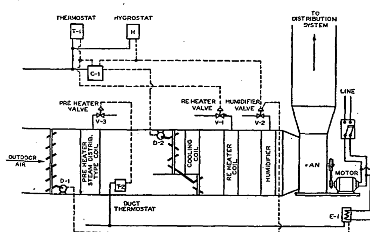
FIG. 2. CONSTANT TEMPERATURE AND HUMIDITY CONTROL FOR YEAR 'ROUND SYSTEM USING 100 PERCENT OUTDOOR AIR
