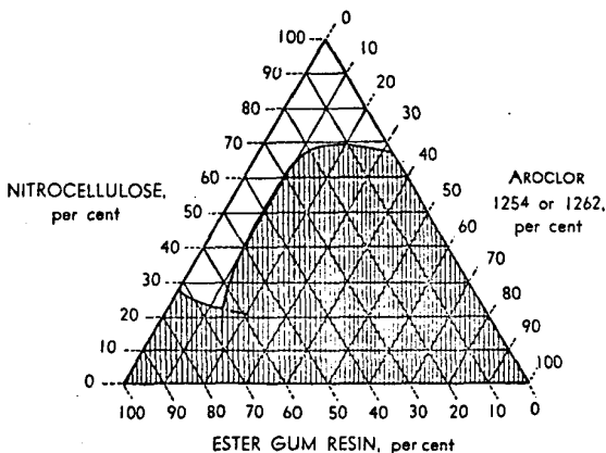
Fig. 1—Limits of Practical Compatibility of AROCLOR in Nitrocellulose Lacquers
