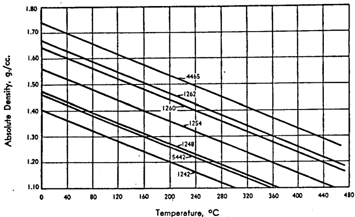
Fig. 2. DENSITIES OF AROCLORS AT VARIOUS TEMPERATURES
