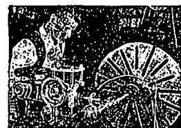
L27 UNIVERSAL METAL WORKER —Versa-Mil drills, boro, mills, faces and grinds (externally, internally and surface). Normally attached to lathe carriage and adjustable at any angle, complete motorized 1-hp unit is easily carried to any job for operation as a self-contained machine tool for maintenance operations on engines, tur-
