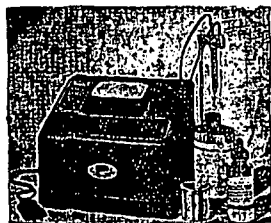
K6 THICKNESS GAGE —Lectroflux is designed for non-destructive inspection and testing of metal containers, vessels and piping while they are in service. Measures steel thickness from 0.125 to 2.250 in. Scott Electroflux Co., Waltham, Mass.
