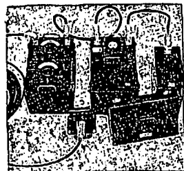
K6 THICKNESS GAGE —Lectroflux is designed for non-destructive inspection and testing of metal containers, vessels and piping while they are in service. Measures steel thickness from 0.125 to 2.250 in. Scott Electroflux Co., Waltham, Mass.
