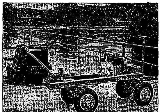
L6 PORTABLE GATE OPERATOR —Power-driven portable gate operator rides on pneumatic-tired wheels. Unit available in three models: electric-motor driven, 5- and 10-hp gasoline engine driven. Princi-
