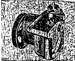
L25 MIDGET HYDRAULIC UNIT —Hydraulic power unit serves many purposes for industrial operations, plant maintenance and service repairs, as arbor press, hydraulic clamping vice, straightening and bending device. It consists of a hydro-power gear pump with hardened and ground gears running in bronze bearings; a compact housing to protect check valves; and a 4-way control valve for operation of double-acting cylinder, hydraulically actuated in either direction. Unit has 3-gpm oil capacity at 1200 rpm, or 4½ gpm at 1800 rpm and 1000 psi. It requires about 2½ hp to operate at 1200 rpm. Equipped with V-belt sheave for driving from fan shaft or power takeoff. Clutch cuts out unit when not in use. Hydraulic Press Mfg Co., Springfield, O.
