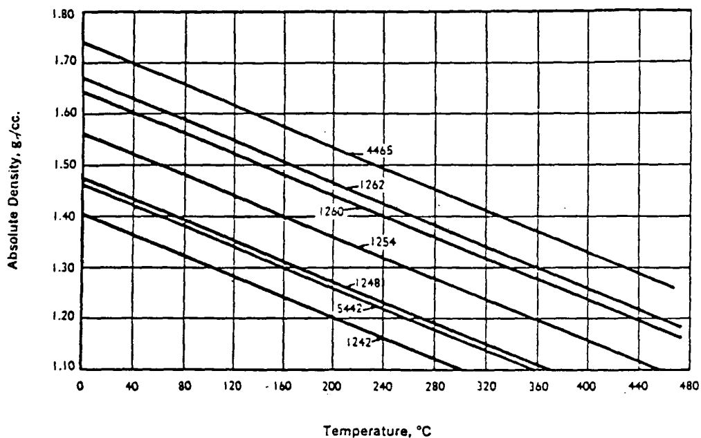
Fig. 1 — Densities of Aroclor® Plasticizers at Various Temperatures
