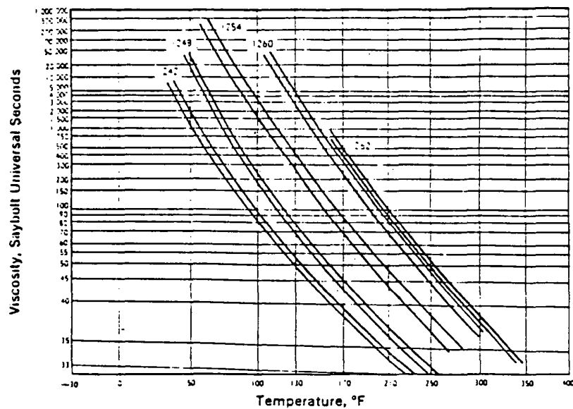
Fig. 3 — Viscosity Ranges of Some Aroclor ® Plasticizers
