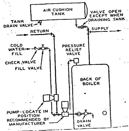
FIG. 16. A CLOSED EXPANSION TANK
