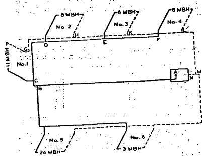
FIG. 13. TWO-PIPE REVERSED RETURN GRAVITY SYSTEM (EXAMPLE 5)
