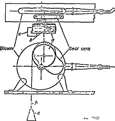
Figure 1.—Apparatus for measuring power required to operate blower. (29 CFR Part 11, Subpart J, § 11.124-2)
