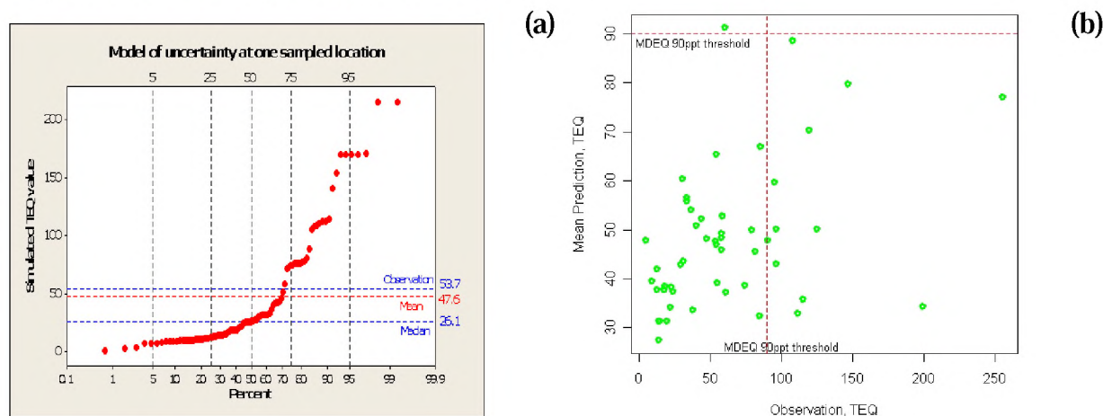
Figure 3. (a) Cumulative distribution of 100 TEQ values simulated at the node the closest to one of the 51 new observations. (b) Scatterplot of observed values versus the mean of the 100 simulated TEQ values (the maximum observation of 923 ppt is not included for graph clarity).
