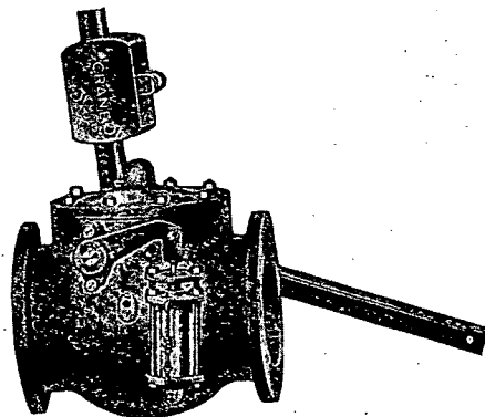
Relief Valve No. 416H Sizes 4 to 36 inch, incl.
