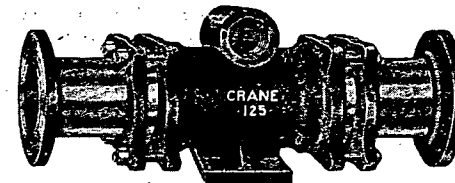
Double Expansion Joint No. 409
