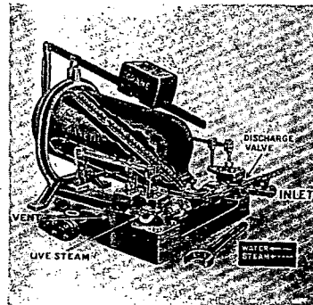
Craneitill 3-Valve Trap Series No. 100 Sizes 1/2 to 3 inch, incl.
