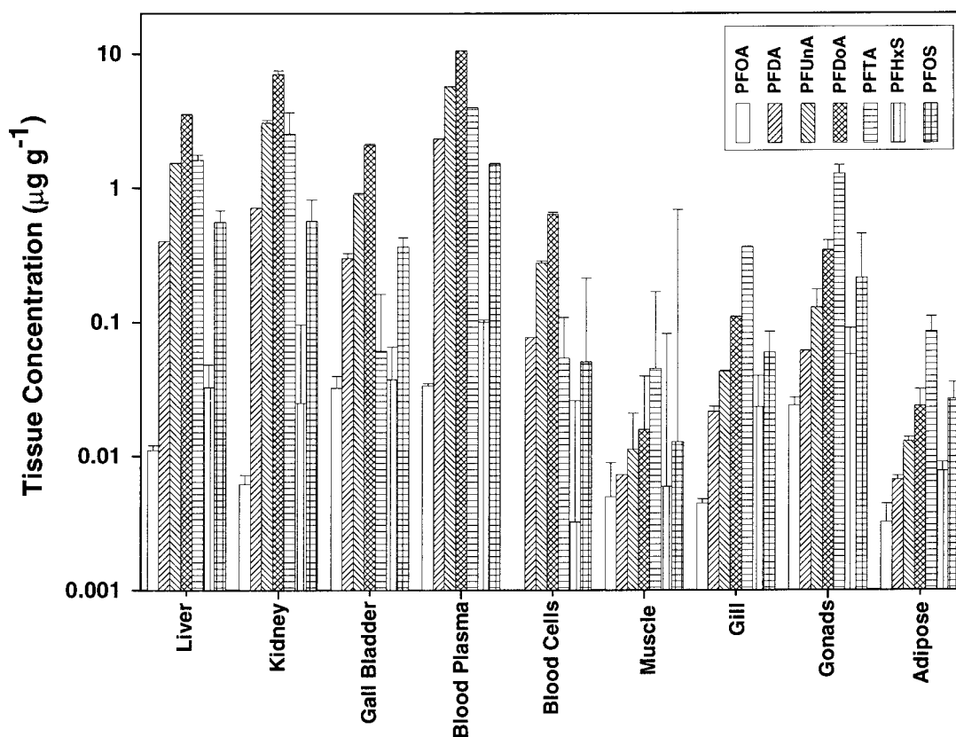
Fig. 2. Perfluorinated acid concentrations, \pm 1 standard error, in various fish tissues after a 12-d aqueous exposure. See Table 1 for definitions of test compounds.
