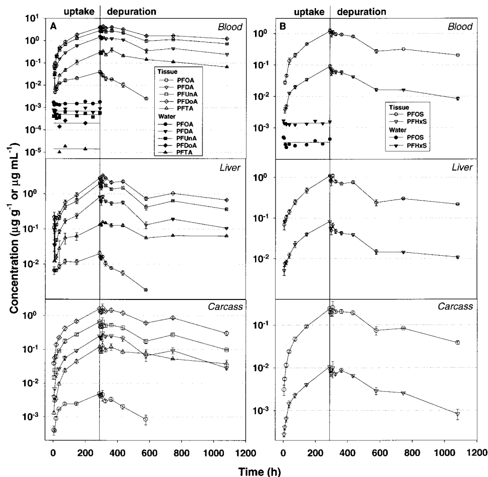
Fig. 1. Growth-corrected uptake and depuration phase concentrations for (A) perfluoroalkyl carboxylates and (B) perfluoroalkyl sulfonates in blood, liver, and carcass. Each tissue concentration represents the mean of three different fish ( \pm 1 standard error). Aqueous exposure concentrations during the uptake phase are shown in A and B for carboxylates and sulfonates, respectively. See Table 1 for definitions of test compounds.
