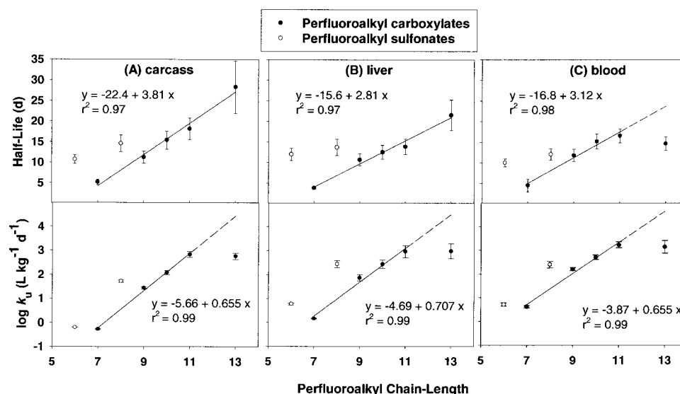
Fig. 3. Half-life ( \ln 2/k_d ) and uptake rate ( \log k_u ) relationships with perfluoroalkyl chain length of carboxylates and sulfonates for (A) carcass, (B) liver, and (C) blood. Linear regression was applied to perfluoroalkyl carboxylate data, and the resulting equation and coefficient of determination ( r^2 ) are shown. The dashed portion of the regression line is an extrapolation and indicates that perfluorotetradecanoic acid was not included in the regression analysis.
