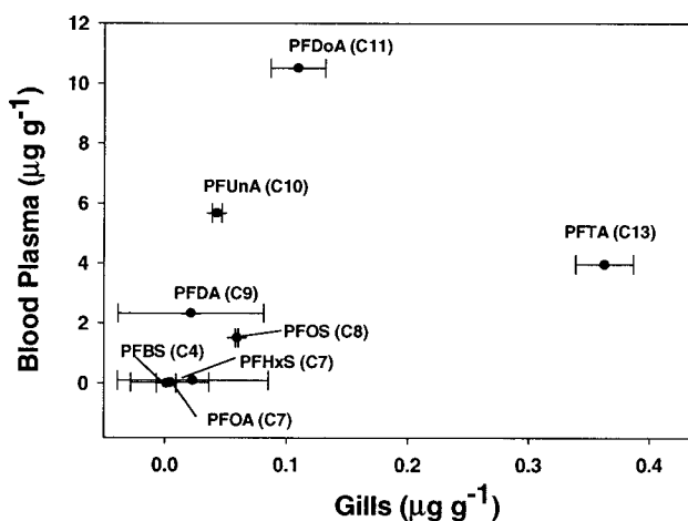
Fig. 4. Relationship between gill and blood concentrations, \pm 1 standard error, in tissue distribution in fish. Each data point represents the mean of three fish, and is labeled with the perfluorinated acid and the length of the respective perfluoroalkyl chain in parentheses (e.g., C8 = eight carbons). See Table 1 for definitions of test compounds.
