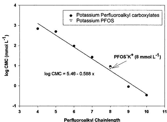
Fig. 6. Relationship determined by linear regression between the log critical micelle concentration (log CMC) and perfluoroalkyl chain length of potassium perfluoroalkyl carboxylate salts. The CMC for the potassium salt of perfluorooctane sulfonate (PFOS- K^+ ) fits the relationship. All data have been taken from Kissa [42].
