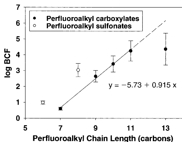
Fig. 5. Carcass bioconcentration factor (BCF) relationship with perfluoroalkyl chain length. Linear regression was applied to perfluoroalkyl carboxylate data, and the resulting equation and coefficient of determination ( r^2 ) are shown. Perfluorotetradecanoic acid was not included in the regression analysis and the dashed portion of the regression line is an extrapolation of the regression equation.
