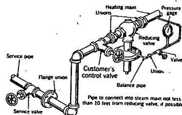
FIG. 2. CONNECTIONS FOR REDUCING VALVE WITHOUT BYPASS
