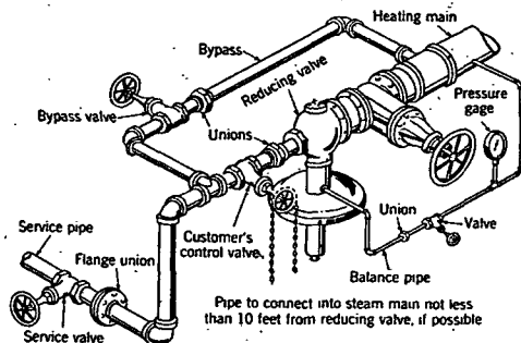
FIG. 3. CONNECTIONS FOR REDUCING VALVE WITH BYPASS
