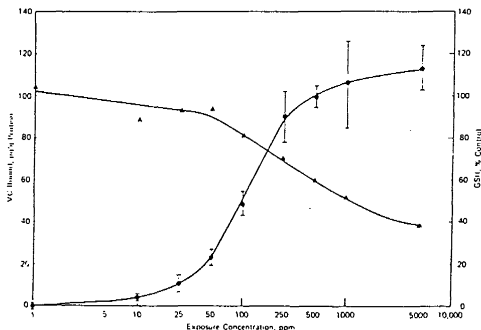
FIG. 1. Hepatic macromolecular binding and glutathione (GSH) depression expressed as a function of the logarithm of the exposure concentration to vinyl chloride (VC). Macromolecular binding ( \bullet ) is expressed as microgram equivalents of VC bound per gram of protein (mean \pm SD). GSH ( \blacktriangle ) is expressed as percentage of control.
