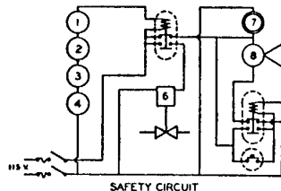
Figure 3. Control and Safety Circuit
