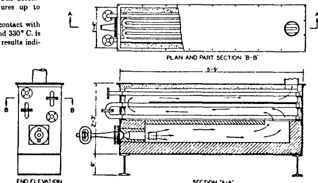
Figure 1. Heater
