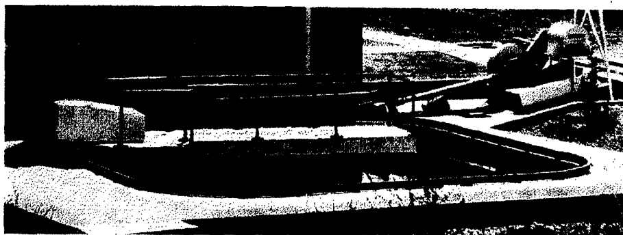
FIGURE 10. DETRITOR, DEVELOPED FROM THE BOWL CLASSIFIER
