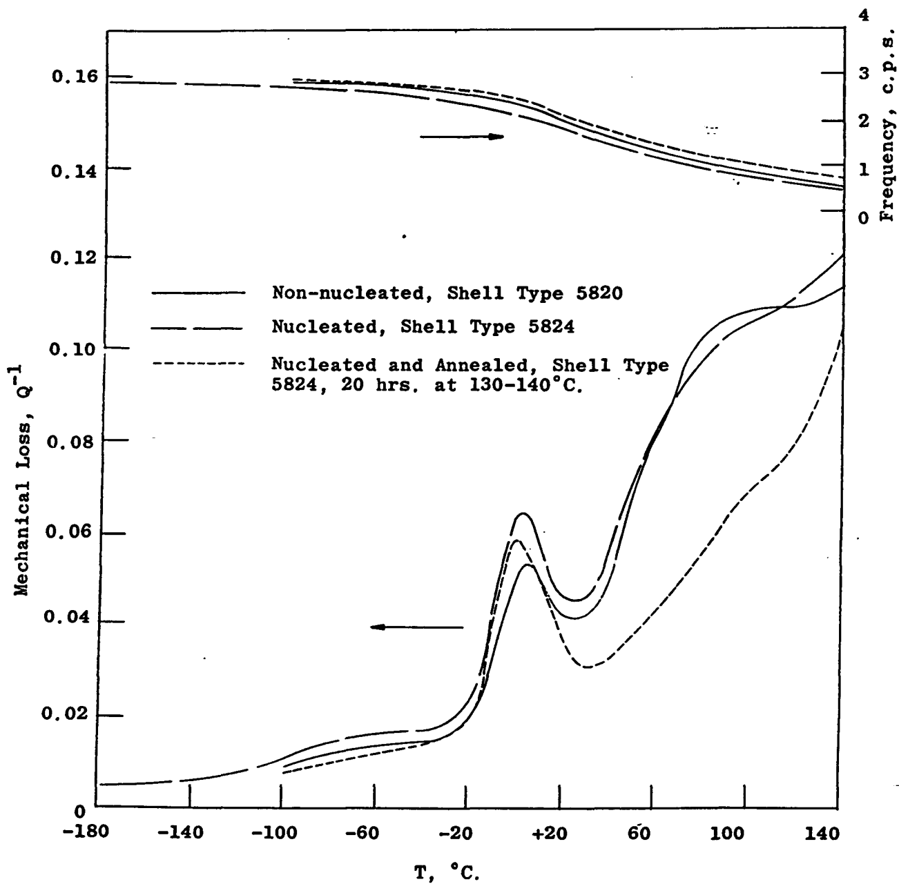
FIGURE 9. MECHANICAL LOSS FOR NON-NUCLEATED AND NUCLEATED POLYPROPYLENE
