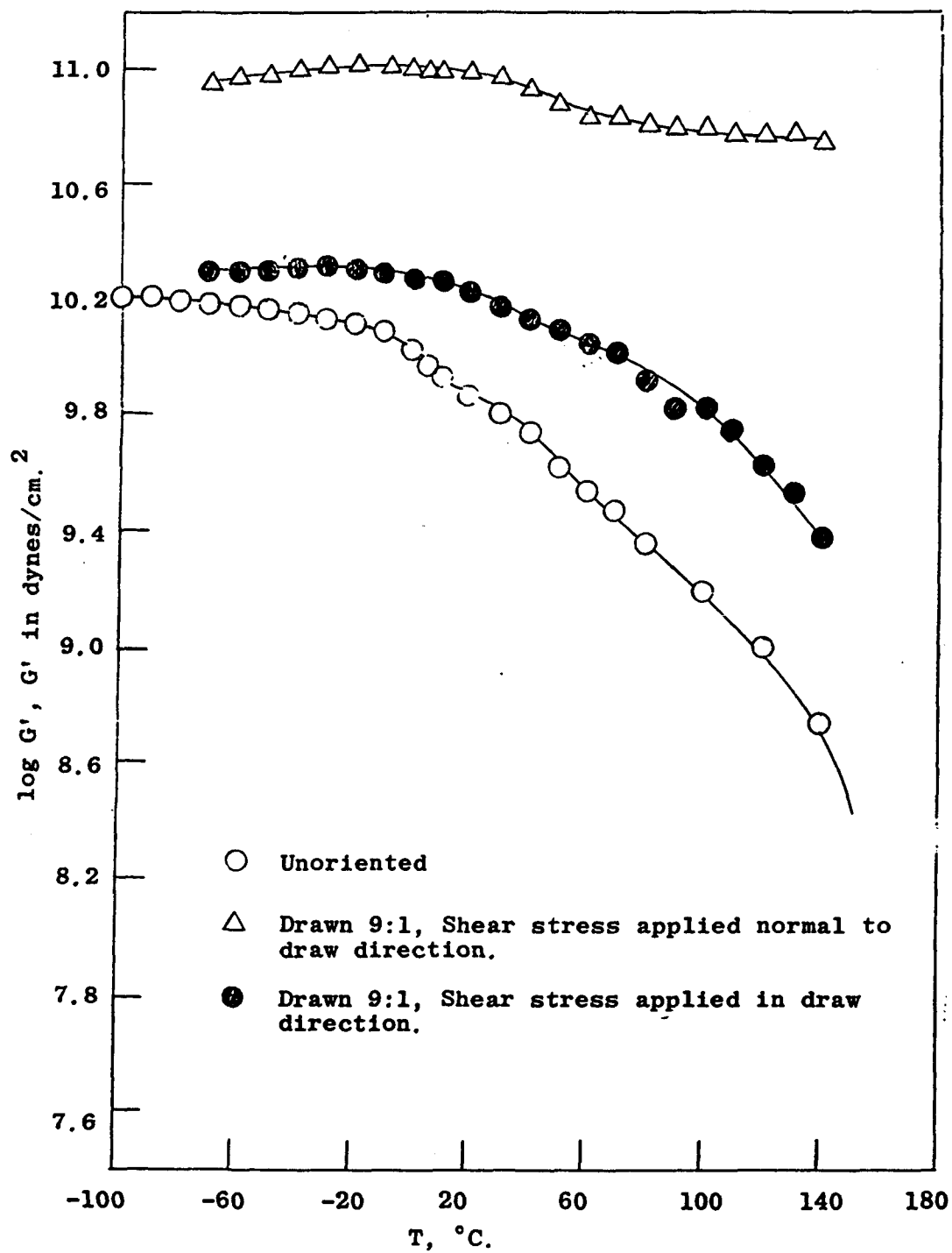
FIGURE 12. REAL COMPONENTS OF THE COMPLEX SHEAR MODULUS FOR UNORIENTED AND ORIENTED SHELL TYPE 5820 POLYPROPYLENE
