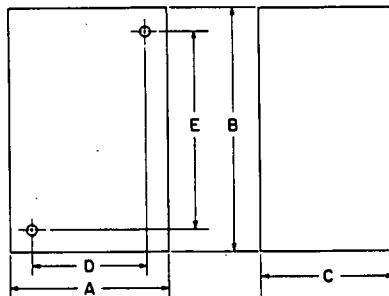
NEMA 1 Surface
