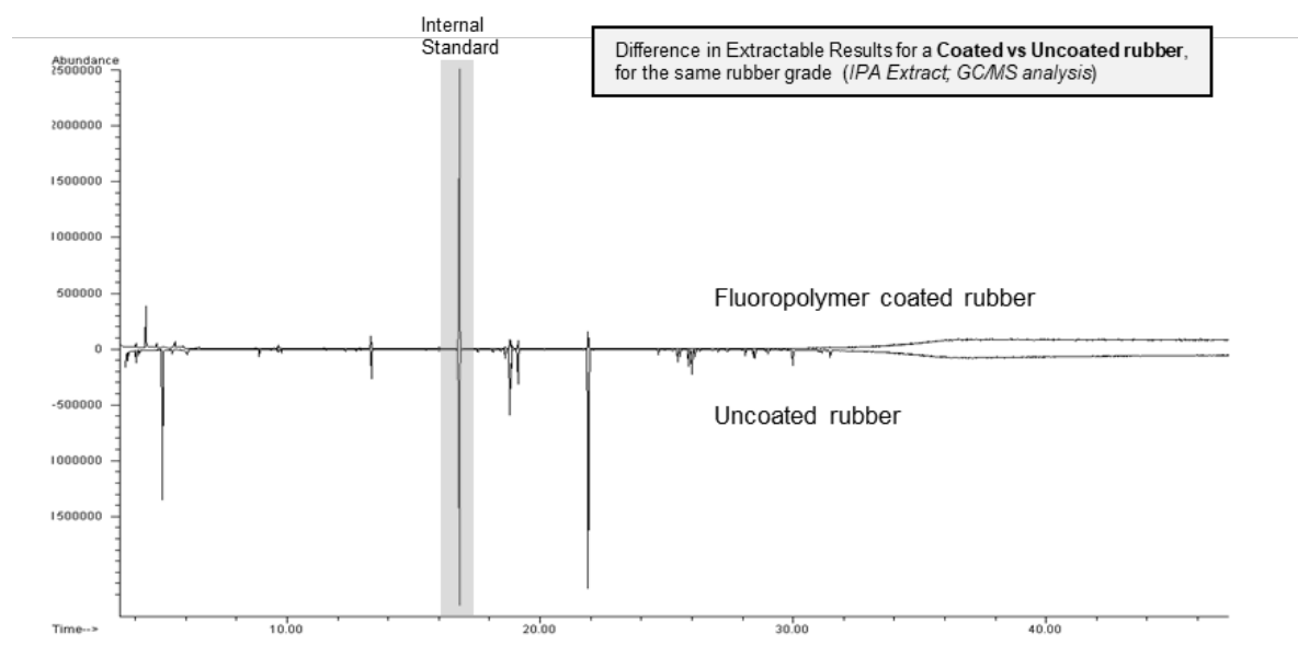
Figure 8: Difference in Extractable Results for a Coated vs Uncoated rubber. Source: ETRMA.
