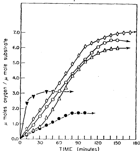
FIG. 2. Rates of oxygen uptake by washed cell suspensions of p -chlorobiphenyl-grown Achromobacter pCB metabolizing various substrates. All rates are corrected for endogenous respiration. (○), p -chlorobiphenyl; (Δ), o -phenylphenol; (▼), catechol; (●), phenylpyruvate; (◇) biphenyl.
