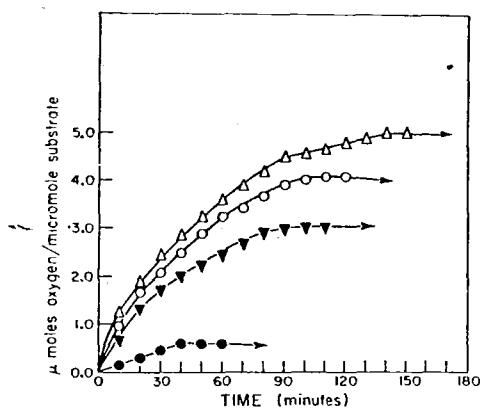
FIG. 4. Rates of oxygen uptake by washed cell suspensions of p -chlorobiphenyl-grown Achromobacter p CB cometabolizing various substrates. All rates are corrected for endogenous respiration. (Δ), o -Chlorobiphenyl; (○), m -chlorobiphenyl; (▼), 4,4'-dichlorobiphenyl; (●), 2,2'-dichlorobiphenyl.
