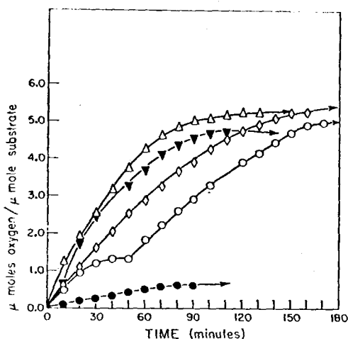
FIG. 3. Rates of oxygen uptake by washed cell suspensions of biphenyl-grown Achromobacter BP cometabolizing various substrates. All rates are corrected for endogenous respiration. ( \diamond ), p -Chlorobiphenyl; ( \Delta ), o -chlorobiphenyl; ( \circ ), m -chlorobiphenyl; ( \nabla ), 4,4'-dichlorobiphenyl; ( \bullet ), 2,2'-dichlorobiphenyl.
