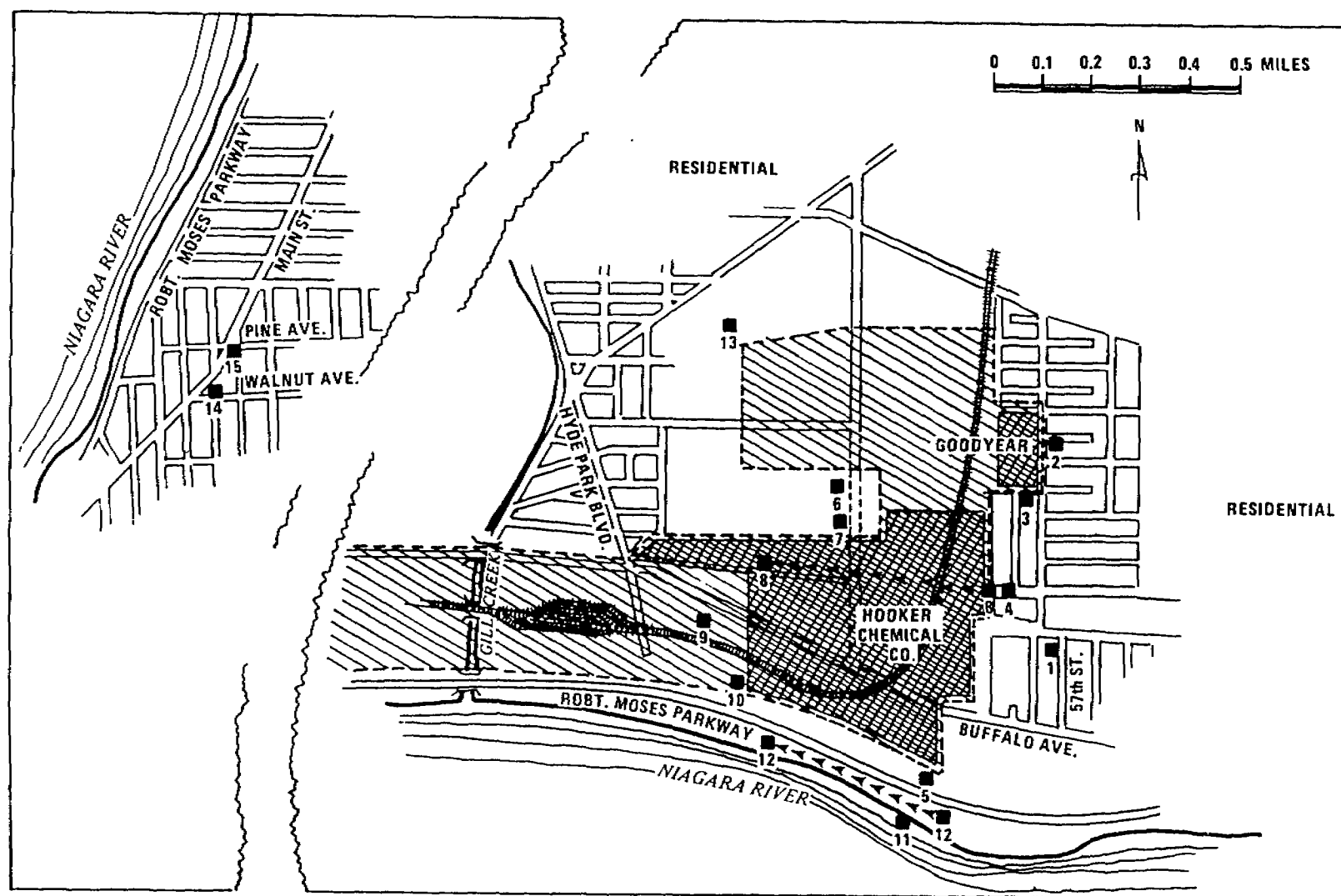
Figure 4.2. Locations of sampling sites for vinyl chloride measurements in Niagara Falls.
