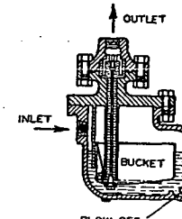
FIG. 26. UPRIGHT BUCKET TRAP
