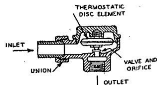
FIG. 24. THERMOSTATIC TRAP DISC TYPE
