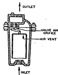
FIG. 27. INVERTED BUCKET TRAP
