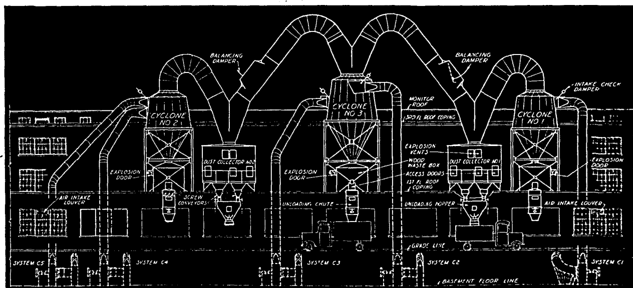
Fig. 3. Elevation showing the external piping, dust collecting equipment, and unloading stations.
