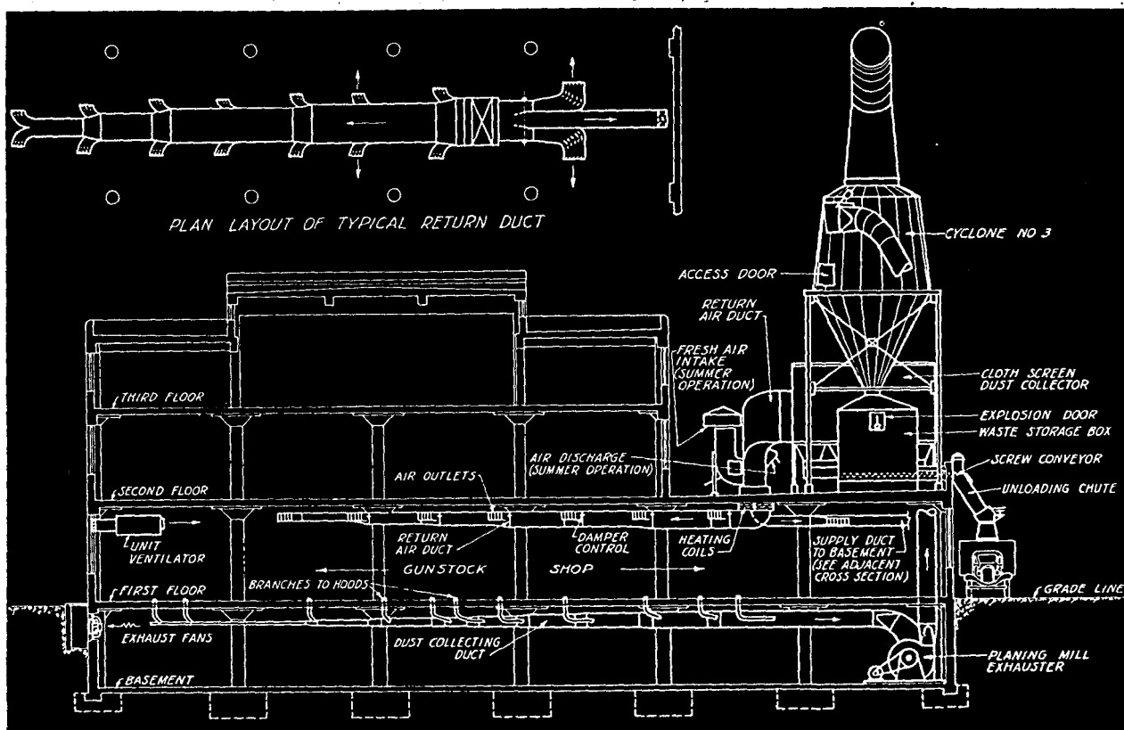
Fig. 2. Cross section showing the arrangement of collecting equipment on roof and relative position of exhaust piping and return ducts; also return duct detail.
