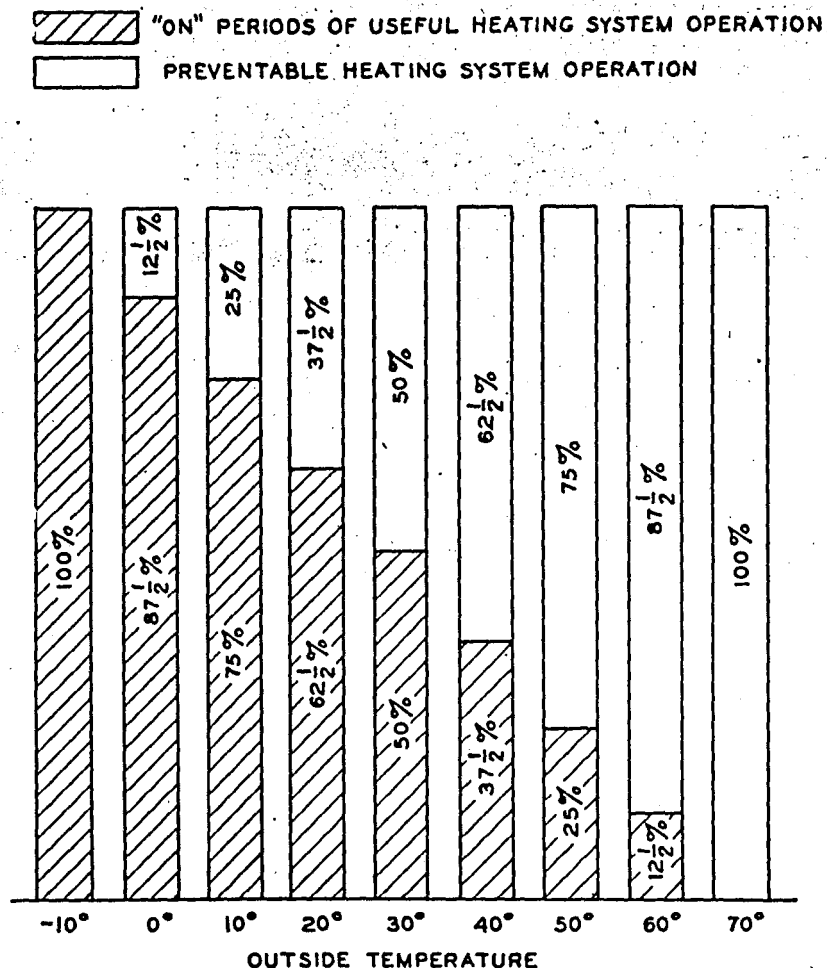
Chart showing "on" and preventable times of heating system operation at various outside temperatures, based on design temperature of -10F.
