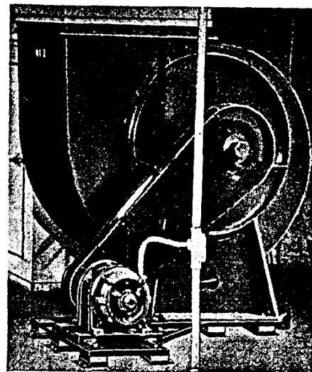
Korfund Girder Type Integral Base installed under large fan and motor. Note how steel girder arrangement provides isolation base common to both fan and motor, thus constantly maintaining essential alignment between them. Compare diagram at left. An economical solution to many machinery installation problems in heating, ventilating and air conditioning. Investigate!
