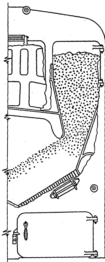
Gravity or magazine feed anthracite-burning boiler, showing coal storage magazine, inclined grate and self-feeding or stoking feature. Coke as a fuel is also recommended.
