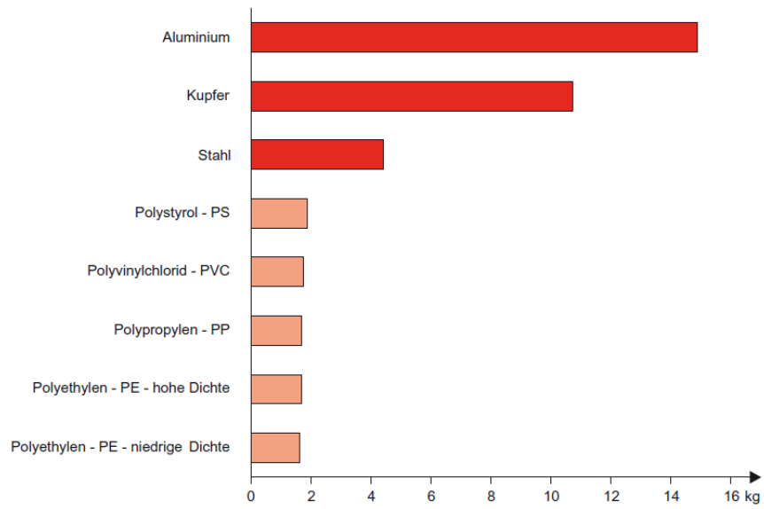
Figure 1: Energy demand measured in kg petroleum consumption / L material volume for the production of materials [Source: Wolfgang Kaiser, Kunststoffchemie für Ingenieure, 4th Newly Edited and Expanded Edition, 2016 Hanser Verlag]
