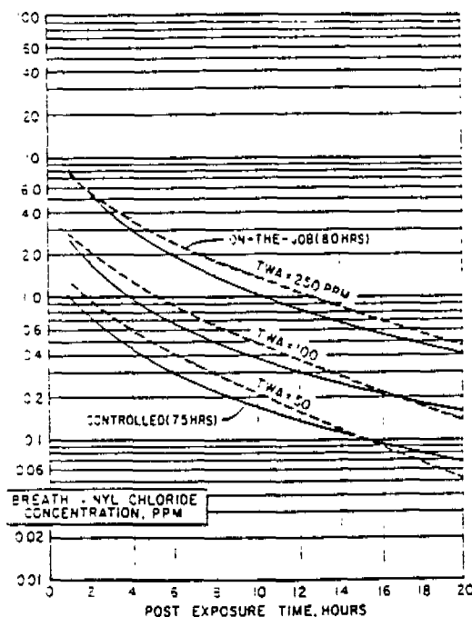
FIGURE 3. Comparison of breath decay curves derived from the on-the-job data and the experimental human exposure data.
