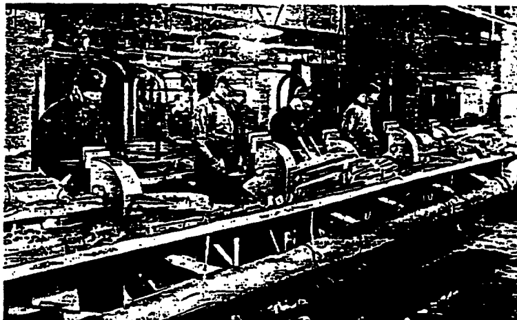
Figure 3. Each of these grinding wheels is partially enclosed by an exhaust hood. Efficient local exhaust is achieved by drawing the dust into the hoods, through branch ducts, and into a control duct which leads to the collection point. (Courtesy American Foundrymen's Society)
