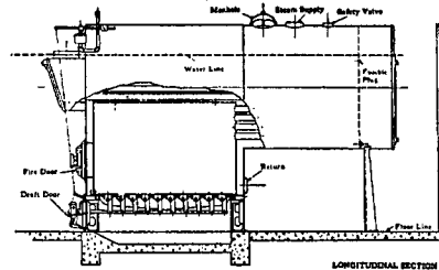
Weld + Rivet Firebox Boiler "5000" Series Up-draft. Also "6000" Series Smokeless Down-draft
