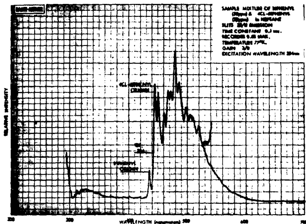
Figure 27. Emission spectrum of a mixture of biphenyl (50 ppm) and 4-chlorobiphenyl (50 ppm) in heptane at 77°K
