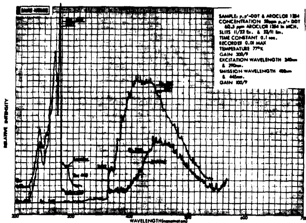
Figure 46. Excitation/emission spectra of a mixture of p,p' -DDT (50 ppm) and Aroclor 1254 (60.5 ppm) in MCH glass at 77°K.
