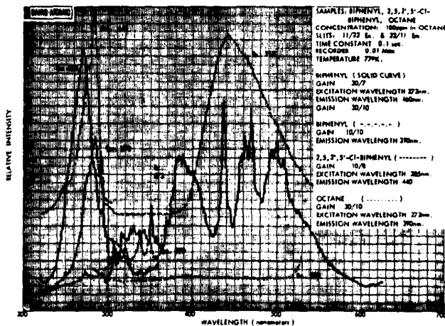
Figure 22. Excitation/emission spectra of biphenyl and 2,5,2',5'-tetrachlorobiphenyl (both 100 ppm) in octane at 77°K
