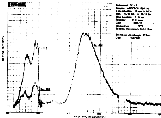
Figure 38 Absorbance/emission spectra of Aracloc 1254 (1% in MCH) at 77°K
