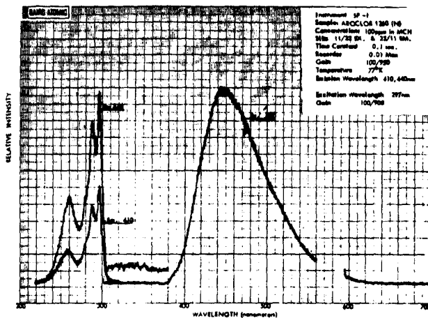
Figure 39. Excitation/emission spectra of Aroclor 1260 (H, 100 ppm) in MCH at 77°K
