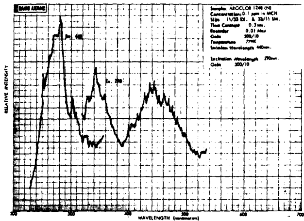
Figure 36. Excitation/emission spectra of Aracloz 1248 (N, 0.1 ppm) in MCH at 77° K
