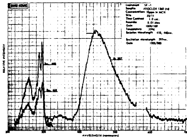
Figure 40. Excitation/emission spectra of Aroclor 1260 (H, 10 ppm) in MCH at 77°K
