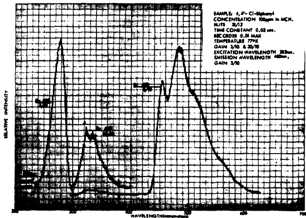
Figure 13. Excitation/emission spectra of 4,4'-dichlorobiphenyl (100 ppm) in MCH glass at 77°K
