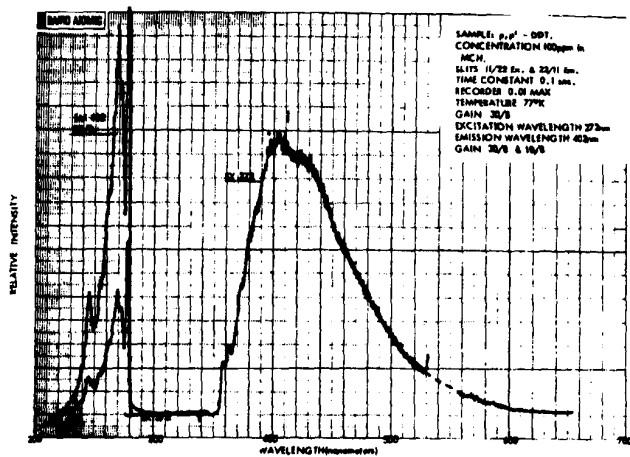
Figure 4. Excitation/emission spectra of p,p'-DDT (100 ppm) in MCH glass at 77° K
