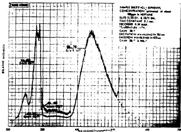
Figure 21. Excitation/mission spectra of 2,4,5,2',5'-pentachlorobiphenyl (100 ppm) in heptane at 77°K.
