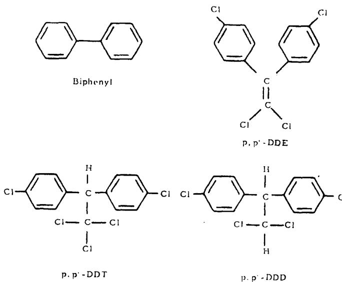
Figure 1. Structural diagrams for biphenyl, p,p'-DDE, p,p'-DDT, and p,p'-DDD
