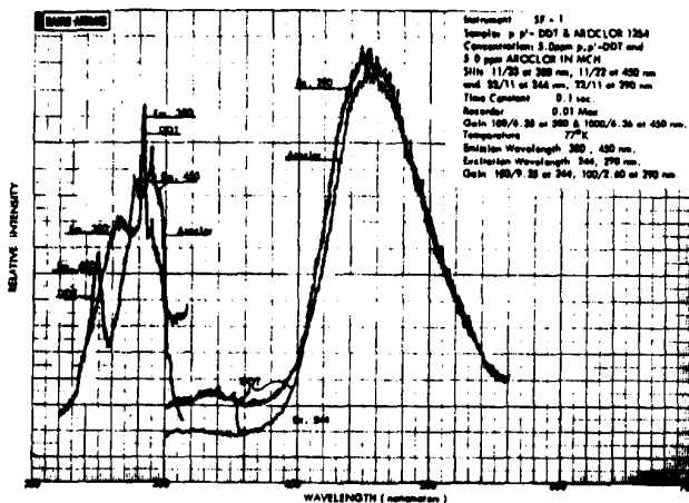
Figure 47. Excitation/emission spectra of a mixture of p,p' -DDT (5 ppm) and Aroclor 1254 (5 ppm) in MCH glass at 77°K.
