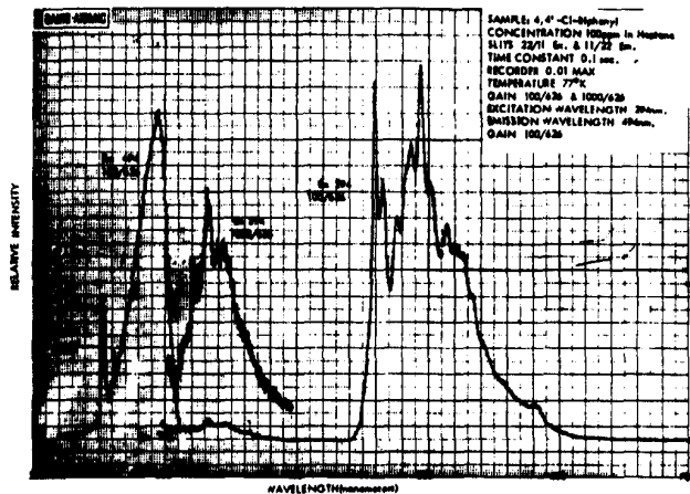
Figure 19. Excitation/emission spectra of 4,4'-dichlorobiphenyl (100 ppm) in heptane at 77°K
