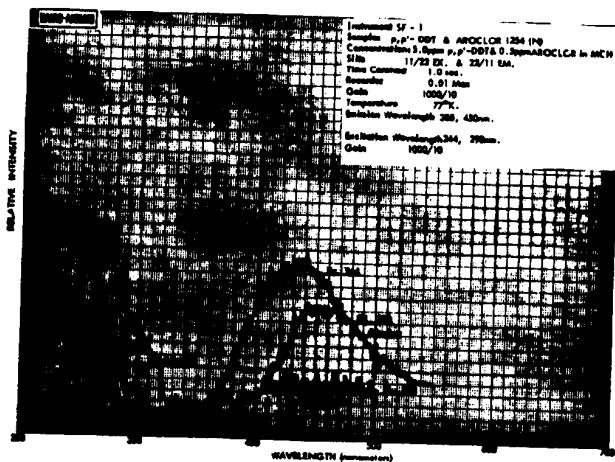
Figure 48. Excitation/emission spectra of a mixture of p,p' -DDT (5 ppm) and Aroclor 1254 (N, 0.5 ppm) in MCH glass at 77°K
