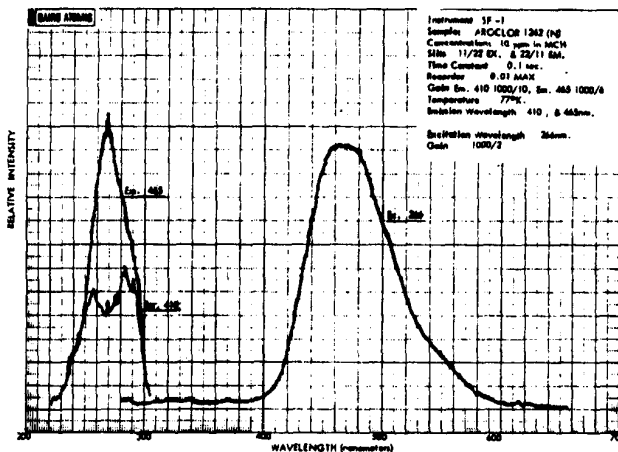
Figure 52. Excitation/emission spectra of Aroclor 1242 (N, 10 ppm in MCH at 77°K)
