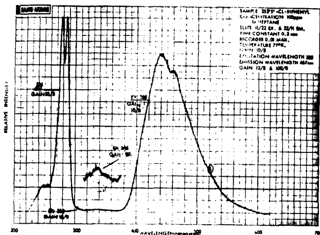
Figure 20. Excitation/mission spectra of 2,4,5,2',5'-tetrachlorobiphenyl (100 ppm) in heptane at 77°K.
