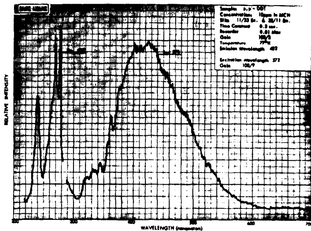
Figure 8. Excitation/emission spectra of p,p' -DDT (10 ppm) in MCH glass at 77^\circ\text{K} .
