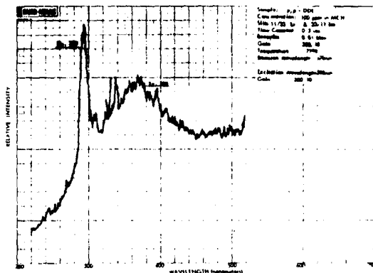
Figure 3. Excitation/emission spectra of p, p'-DDE (100 ppm) in methylcyclohexane (MCH) glass at 77° K
