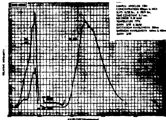
Figure 28. Excitation/emission spectra of Aroclor 1254 (100 ppm) in MCH glass at 77° K
