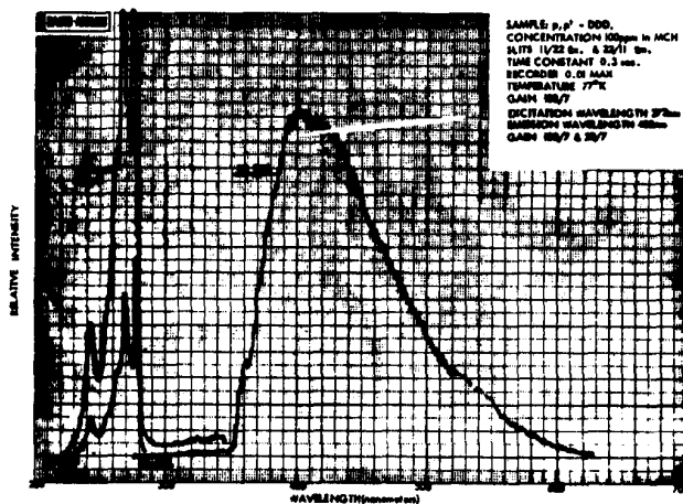
Figure 6. Excitation/emission spectra of p,p' -DDD (100 ppm) in MCH glass at 77°K
