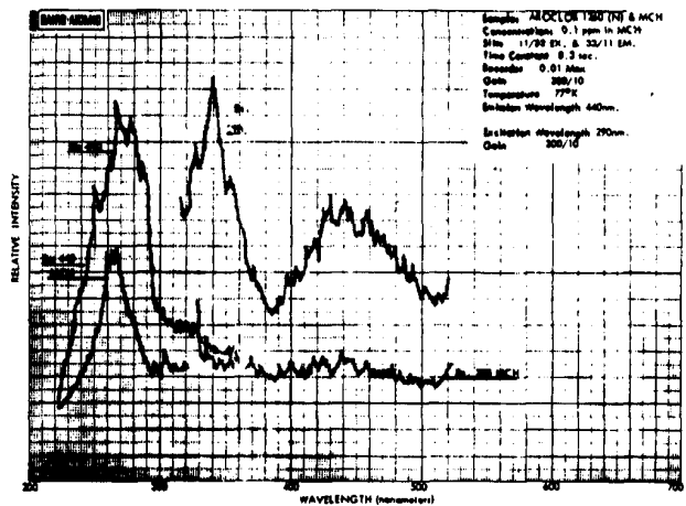
Figure 42. Excitation/emission spectra of Aracloz 1260 (N, 0.1 ppm) in MCH at 77° K
