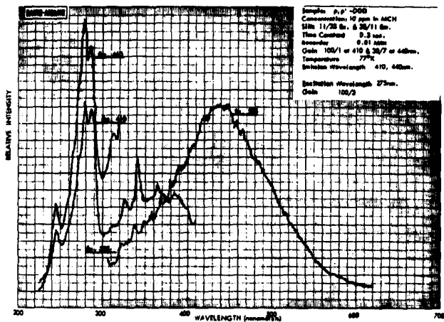
Figure 10. Excitation/emission spectra of p,p' -DDD (10 ppm) in MCN glass at 77°K.
