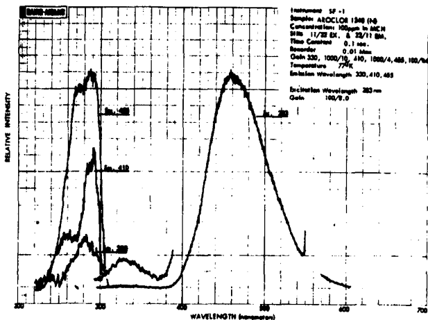
Figure 33. Excitation/emission spectra of Araclo 1248 (N, 100 ppm) in MCH at 77°K
