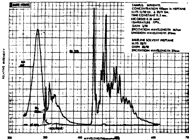
Figure 16. Excitation/emission spectra of biphenyl (100 ppm) in heptane at 77°K
