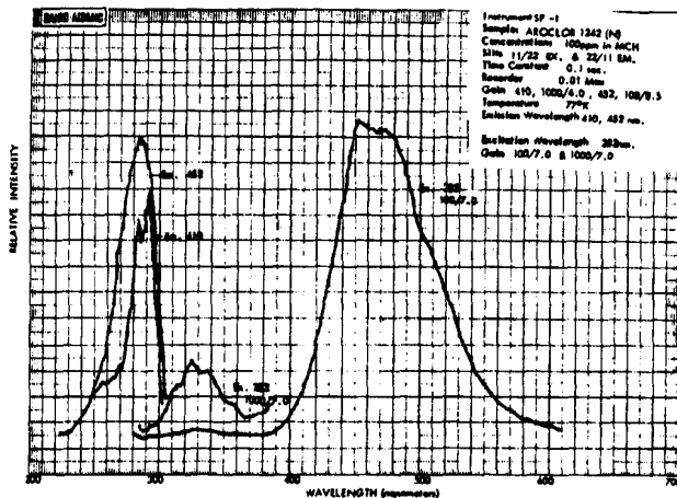
Figure 51. Excitation/emission spectra of Aroclor 1242 (N, 100 ppm in MCH at 77°K)
