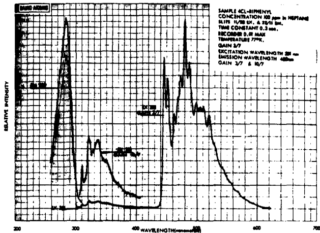
Figure 18. Excitation/emission spectra of 4-chlorobiphenyl (100 ppm) in heptane at 77°K
