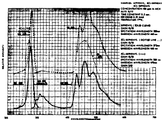
Figure 12. Excitation/emission spectra of biphenyl, 2-chlorobiphenyl, and 4-chlorobiphenyl (all 100 ppm) in MCH glass at 77°K
