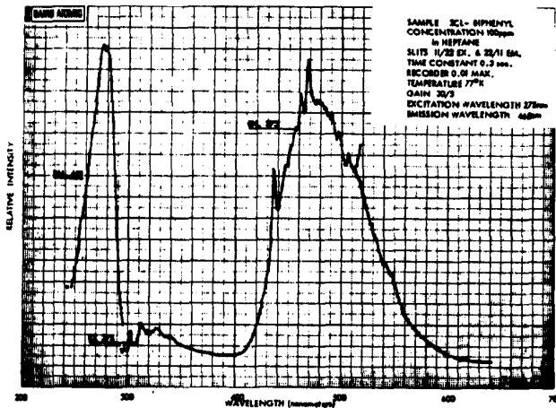
Figure 17. Excitation/emission spectra of 2-chlorobiphenyl (100 ppm) in heptane at 77°K
