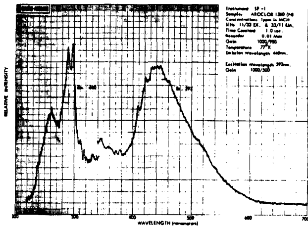
Figure 41. Excitation/emission spectra of Aracloz 1260 (N, 1 ppm) in MCH at 77° K
