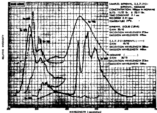
Figure 23. Excitation/emission spectra of biphenyl and 2,5,2',5'-tetrachlorobiphenyl (both 100 ppm) in nonane at 77°K
