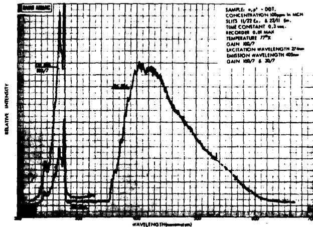
Figure 5. Excitation/emission spectra of o,p'-DDT (100 ppm) in MCH glass at 77° K
