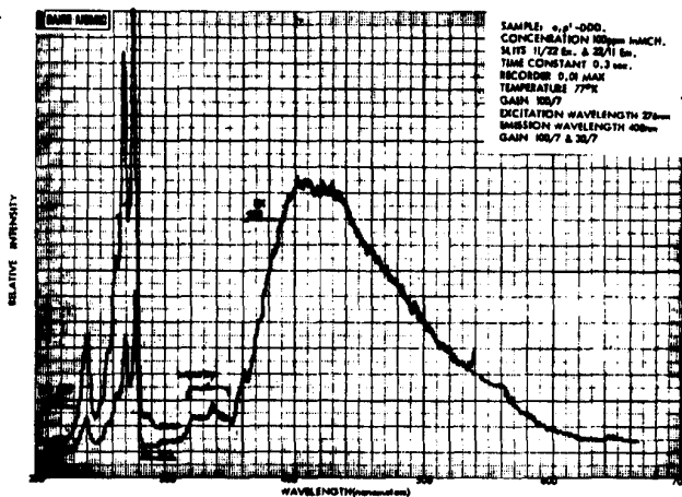
Figure 7. Excitation/emission spectra of o,p' -DDD (100 ppm) in MCH glass at 77°K
