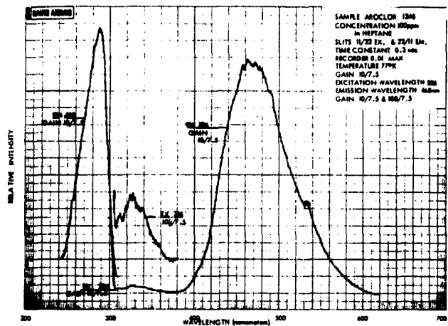
Figure 25. Excitation/emission spectra of Aroclor 1248 (100 ppm) in heptane at 77° K
