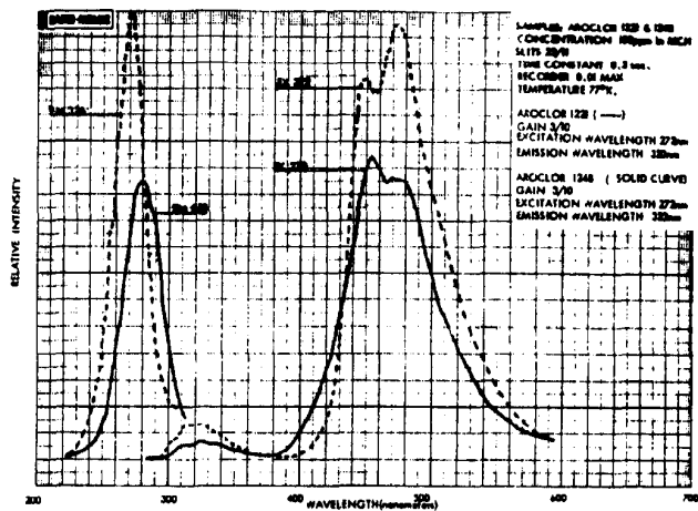
Figure 24. Excitation/emission spectra of Aroclor 1221 and 1248 (both 100 ppm) in MCH glass at 77° K
