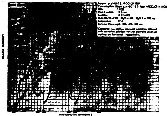
Figure 50. Polarized excitation spectra of a mixture of Aroclor 1254 (5 ppm) and p, p' -DDT (50 ppm) in MCH glass at 77^\circ \text{K}
