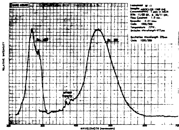
Figure 35. Excitation/emission spectra of Aracloz 1248 (N, 1 ppm) in MCH at 77° K
