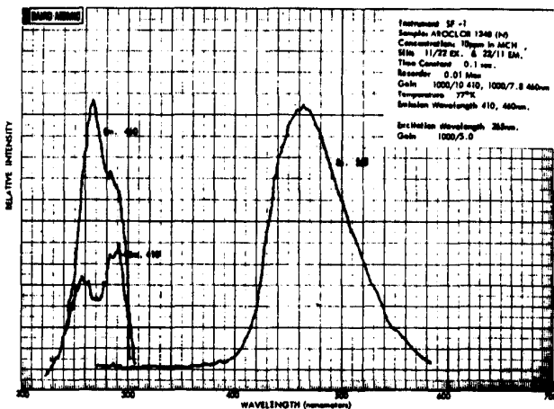
Figure 34. Excitation/emission spectra of Araclo 1248 (N, 10 ppm) in MCH at 77°K
