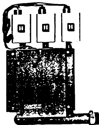
Illustrated is Comfort Computer-Zone Valve Package
