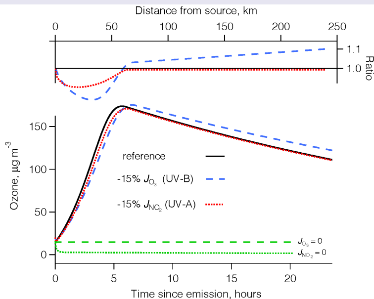
Box 3. Illustration of the response of ground-level ozone to changes in J_{\text{O}_3} (mostly UV-B) and J_{\text{NO}_2} (mostly UV-A), calculated with a simplified kinetic model. Ozone is produced rapidly near sources of pollution (e.g., cities), but is destroyed slowly as air parcels are transported away by winds (taken here as 10 \text{ km h}^{-1} ). Less intense UV-A radiation generates less ozone initially but not at later times. Less intense UV-B radiation leads to even less initial production of \text{O}_3 , but also to a slower decrease at longer times. The lower panel shows \text{O}_3 concentrations, while the upper panel shows the changes as ratios to the reference. Values of the maximum in \text{O}_3 concentration and its timing are illustrative only, with actual values sensitive to the spatial and temporal patterns of emissions, the chemical nature of the emissions, day/night cycles, and details of meteorological transport. The reference chemical mechanism is: \text{O}_3 + \text{UV-B} \rightarrow 2\text{OH} ( 7 \times 10^{-6} ); \text{OH} + \text{RC} \rightarrow \text{HO}_2 ( 10^{-11} ); \text{HO}_2 + \text{NO} \rightarrow \text{OH} + \text{NO}_2 ( 8.1 \times 10^{-12} ); \text{O}_3 + \text{NO} \rightarrow \text{NO}_2 ( 1.9 \times 10^{-14} ); \text{NO}_2 + \text{UV-A} \rightarrow \text{NO} + \text{O}_3 ( 10^{-2} ); \text{NO}_2 + \text{OH} \rightarrow \text{HNO}_3 ( 1.1 \times 10^{-11} ); 2\text{HO}_2 \rightarrow \text{H}_2\text{O}_2 ( 2.90 \times 10^{-12} ), with rate coefficient units of \text{s}^{-1} for photolysis and \text{cm}^3 \text{ molec}^{-1} \text{ s}^{-1} for bimolecular reactions, and initial concentrations of \text{O}_3 ( 20 \mu\text{g m}^{-3} ), \text{NO} ( 12.5 \mu\text{g m}^{-3} ), and \text{RC} ( 10 \times \text{NO} , molar basis).
