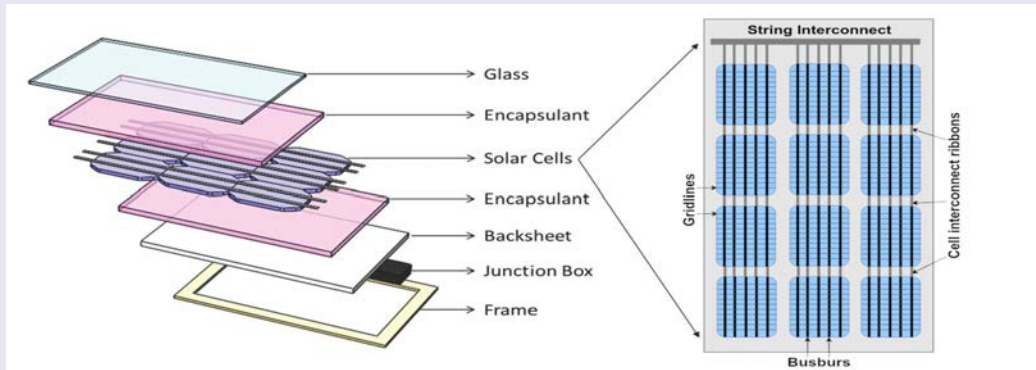
Fig. 4 Components of a crystalline silicon photovoltaic (PV) module illustrating the placement of encapsulants and backsheet, both made of plastic materials prone to degradation by solar UV radiation (modified from [187]).
