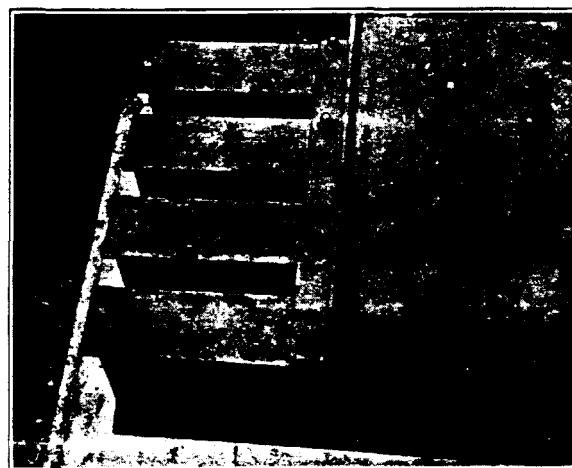
A lead-asbestos anti-vibration pad under a grillage of the new Waldorf-Astoria Hotel
