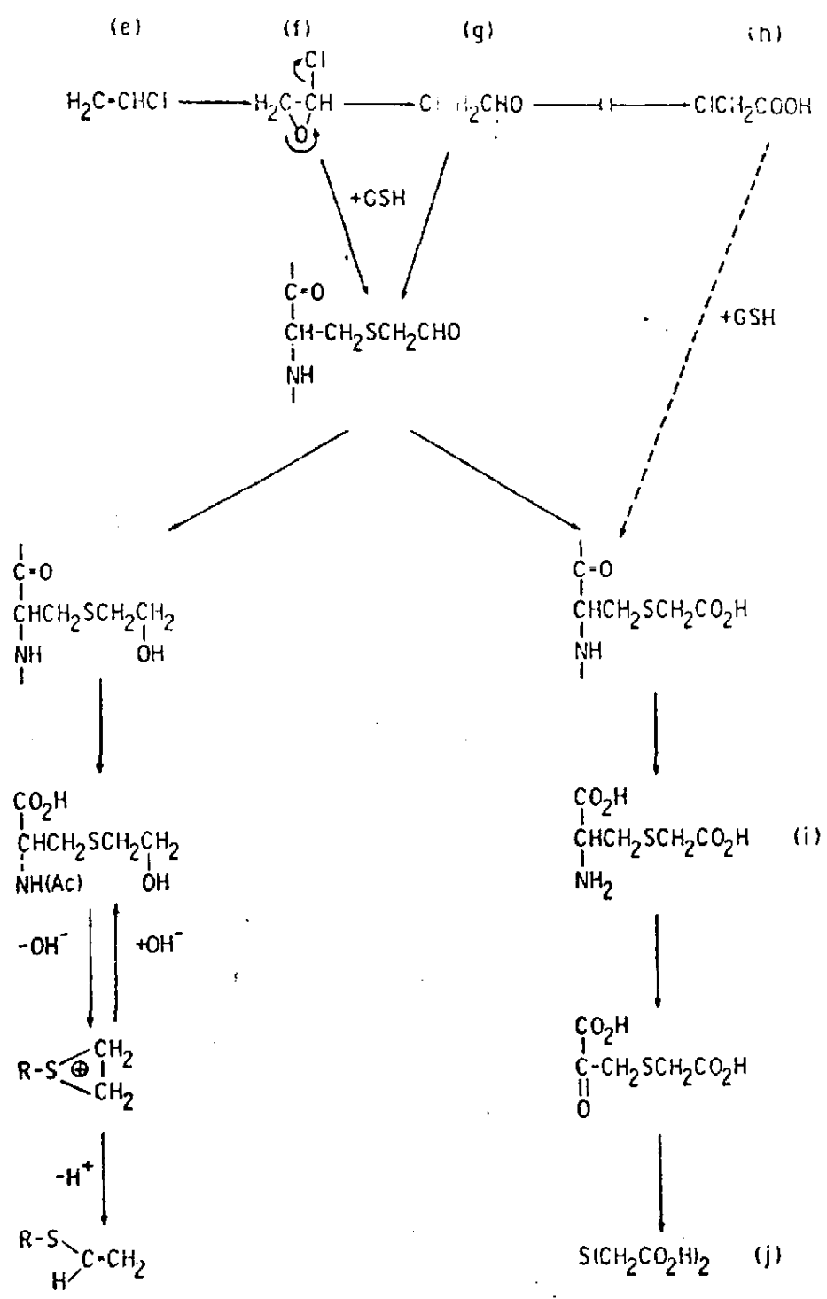
Fig. 3 Scheme for the biogenesis of S -containing vinyl chloride metabolites
