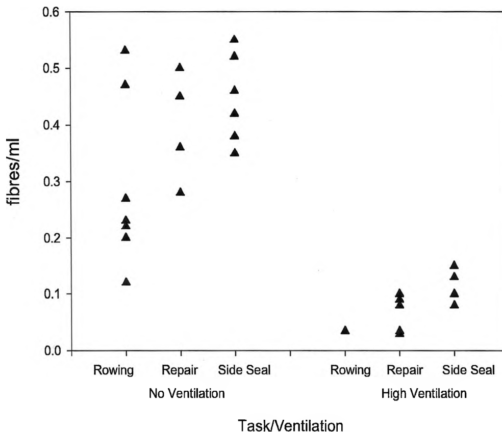
Figure 1 Fibre exposure levels during simulated work with asbestos mitts.
