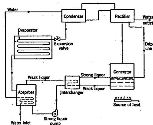
FIG. 7. CLOSED ABSORPTION SYSTEM
