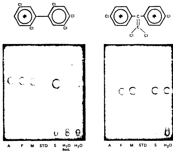
Fig. 2C. Radioautogram of TLC plate containing extracts of water and organisms treated with 2,4,5,2',5'-pentachlorobiphenyl. A (alga), F (fish), M (mosquito larva), S (snail) and STD ( 14 C-radiolabeled compound).
