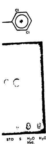
Fig. 2C. Radioautogram of TLC plate containing extracts of water and organisms treated with 2,4,5,2',5'-tetrachlorobiphenyl. A (alga), F (fish), M (mosquito larva), S (snail) and STD ( 14 C-radiolabeled compound).
