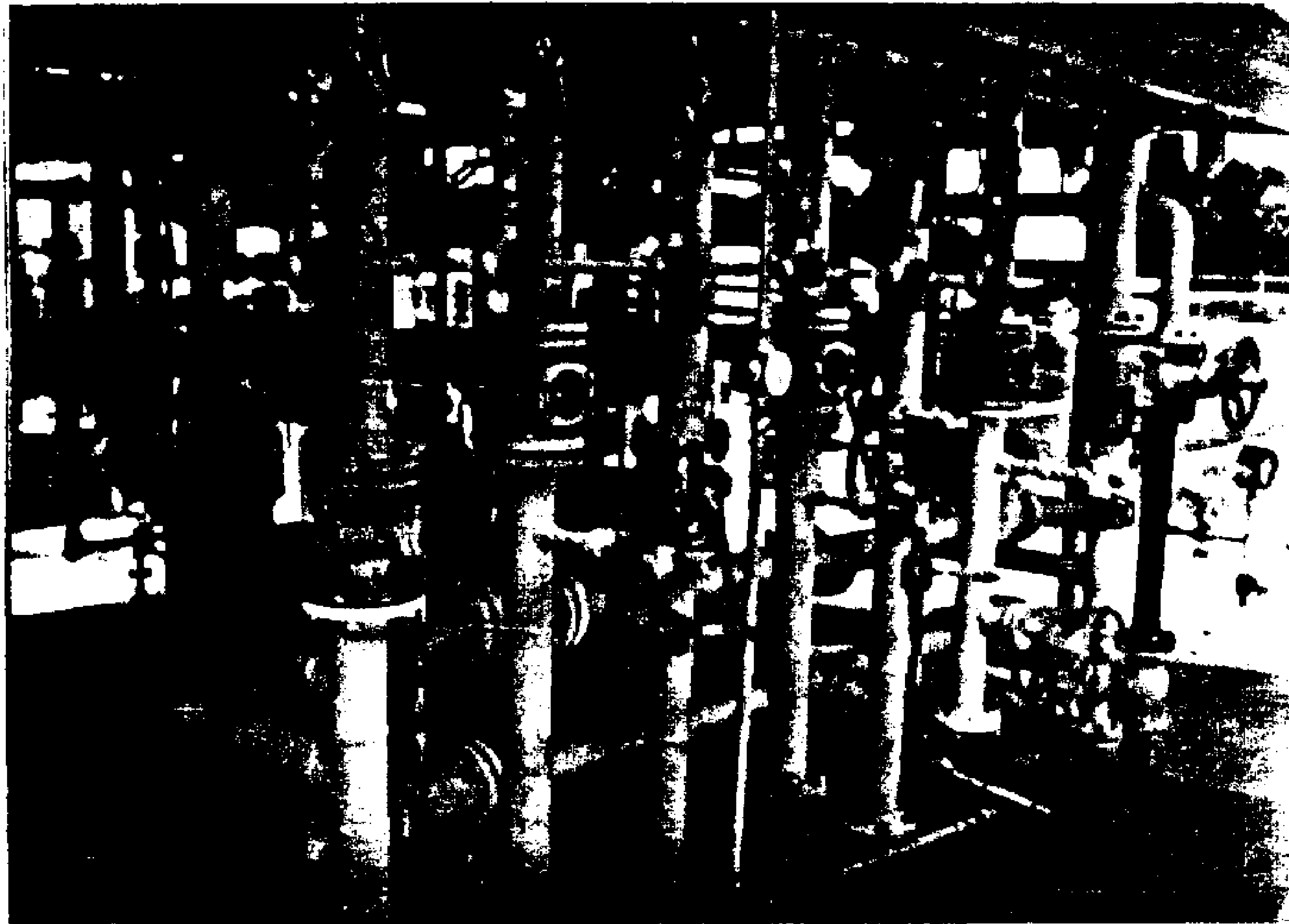
FIG. 5 - SIGHT GLASSES FOR CHECKING VCM LIQUID UNLOADING, LOCATED ON EAST SIDE OF COMPRESSOR SHED
