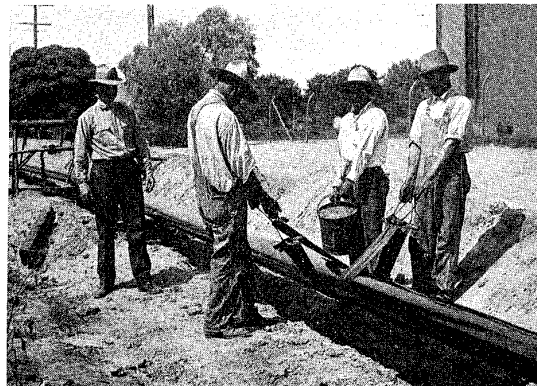
APPLICATION OF "McEVERLAST" ELECTROLYSIS PROOF COATING TO 8-INCH GAS MAIN OF SOUTHERN CALI- FORNIA GAS COMPANY
