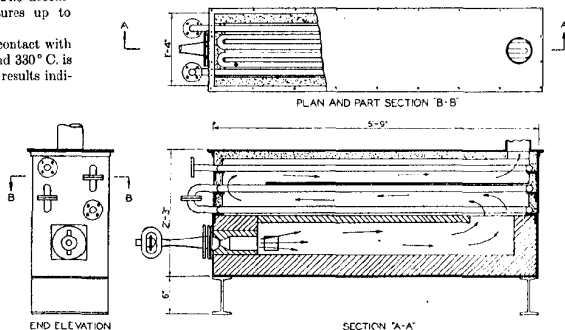
Figure 1. Heater
