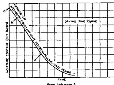
Fig. 1 . . . Moisture Content w vs. Drying Time \theta
