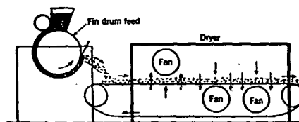
FIG. 14. SECTION OF CONTINUOUS DRYER, BLOW-THROUGH TYPE
