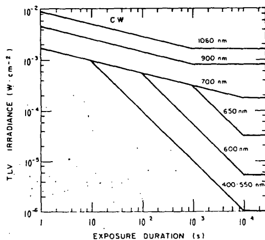
Figure 3a — TLV for infrabeam (direct) viewing of CW laser beam (400-1400 nm)
