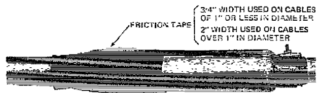
Friction Tape Wrapping Applied to Joint
