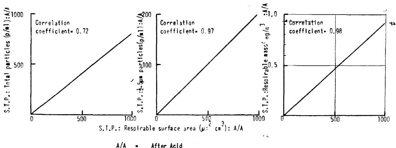
Fig. 2—Conversion between various dust measures
