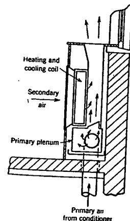
FIG. 11. INDUCTION UNIT (HIGH PRESSURE TYPE)
