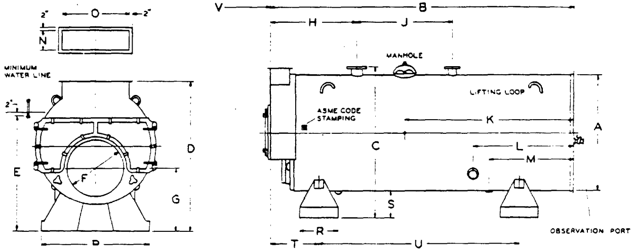
dimensions and data (feet—inch)
