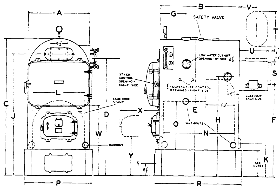
dimensions and data (feet-inches)
