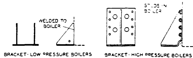
BRACKET - LOW PRESSURE BOILERS
