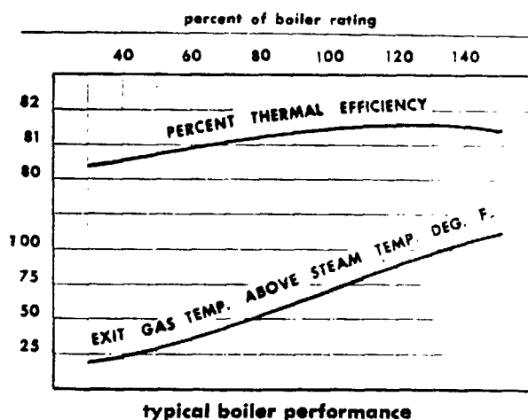
typical boiler performance
