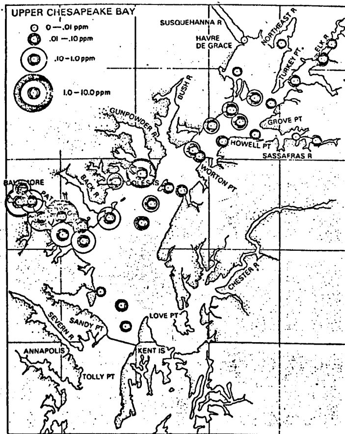
Figure 4. A representation of the concentration of PCB's in bottom sediments samples from the upper Chesapeake Bay.
