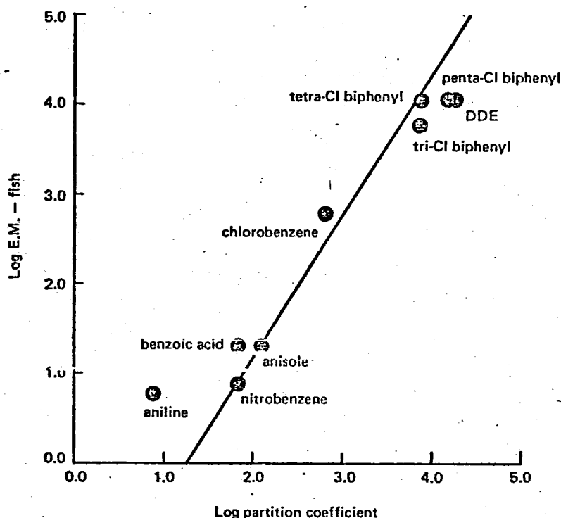
Fig. 5. Plot of log E.M. (ecological magnification) for fish vs. log octanol/water partition coefficient.
