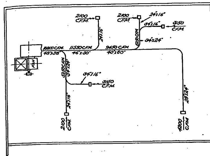
FIG. 7. EXHAUST SYSTEM LAYOUT
