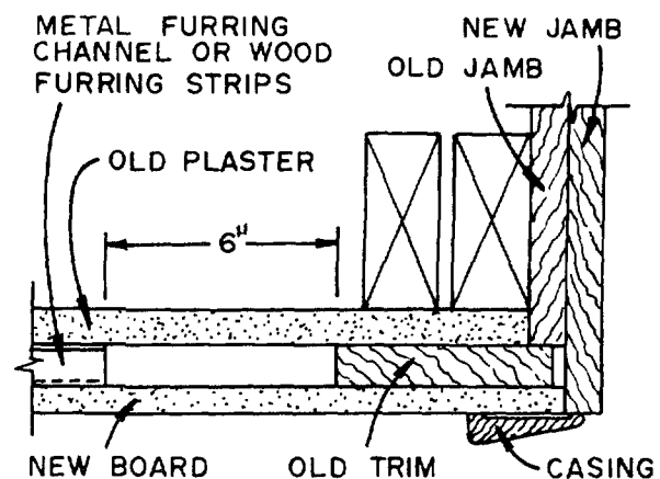
Figure 6—Door Framing Detail with New Casing.
