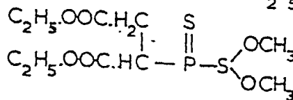
Fig. 14.—Formulae of active compounds in organo-phosphorus insecticides.
