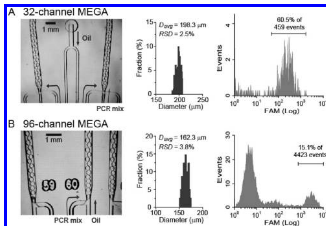
Figure 3. Characterization of droplet generation and PCR amplification using MEGAs. (A) 32-channel MEGA chip. Left: photo of the cross-shaped nozzles each generating \sim 4 \text{ nL} droplets at 5.6 Hz ( 6.4 \times 10^5 droplets per hour). Middle: size distribution of uniform droplets collected from eight nozzles in a device. RSD: relative standard deviation. Right: a representative flow cytometric analysis of 624 bp amplicons on beads amplified from pUC18 template (1 copy/droplet) in \sim 3 \text{ nL} droplets generated from four nozzles in a device. (B) 96-channel MEGA. Left: image of droplet production at the T-shaped nozzles with a total throughput of 2.4 \times 10^6 droplets per hour. Middle: size distribution of uniform \sim 2 \text{ nL} droplets collected from 16 nozzles in a device. Right: a representative flow cytometric histogram of beads carrying the FAM labeled PCR product from E. coli K12 at 0.2 cells per droplet (cpd) in 2.5 nL droplets. For all tests of droplet generation, the mock PCR mix containing \sim 100 beads per \mu\text{L} was used.
