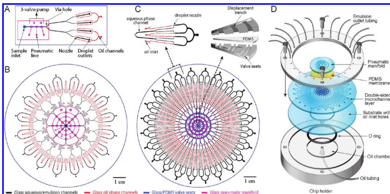
Figure 2. Microfluidic emulsion generator array (MEGA) devices. (A) Layout of a glass/PDMS/glass hybrid four-channel MEGA device with a pneumatically controlled three-valve micropump integrated to drive four nozzles for droplet generation. (B) Design of a 32-channel MEGA device using an array of eight identical micropumps to operate 32 nozzles simultaneously. Two adjacent emulsion channels are combined to increase device density. (C) Layout of 96-channel MEGA on a 4 in. wafer composed of a single ring pump and 96 droplet generators. Inset: close-ups of a single repeating unit composed of four T-shaped nozzles (left) and the pump structure schematically showing three pairs of coaxial ring-shaped valves and displacement trenches (right). (D) Exploded view of the complete four-layer 96-channel MEGA device and the plexiglass assembly module used to infuse oil and to collect the generated emulsion.
