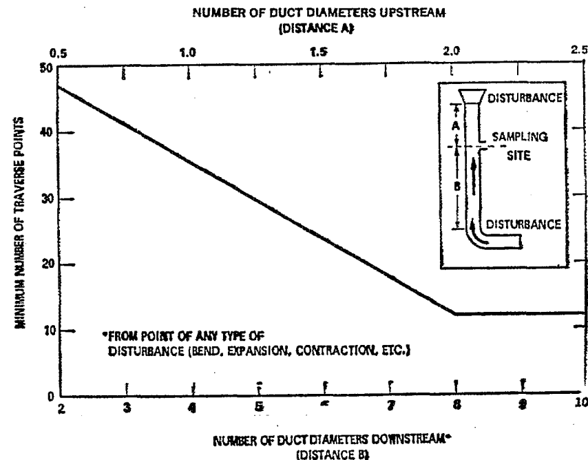
Figure 102-3. Minimum of traverse points.
