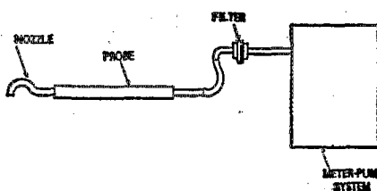
Figure 103-1. Beryllium screening method: sample train schematic.
