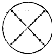
Figure 102-4. Cross section of circular stack showing location of traverse points on perpendicular diameters.
