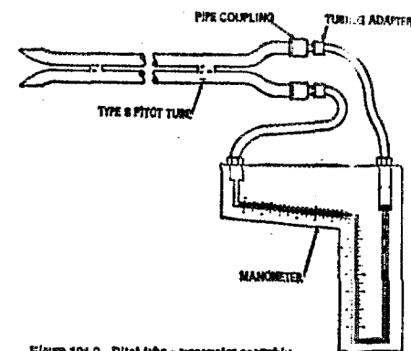
Figure 101-2. Pitot tube - manometer assembly.
