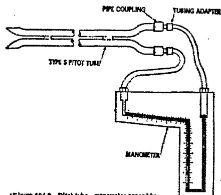
Figure 104-2. Pitot tube - manometer assembly.
