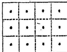
Figure 101-5. Cross section of rectangular stack divided into 12 equal areas, with traverse points at centroid of each area.
