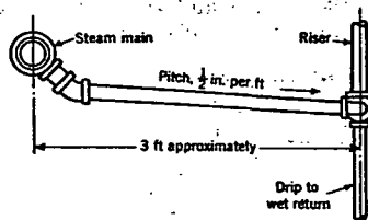
FIG. 7. TYPICAL STEAM RUNOUT WHERE RISERS ARE DRIPPED
