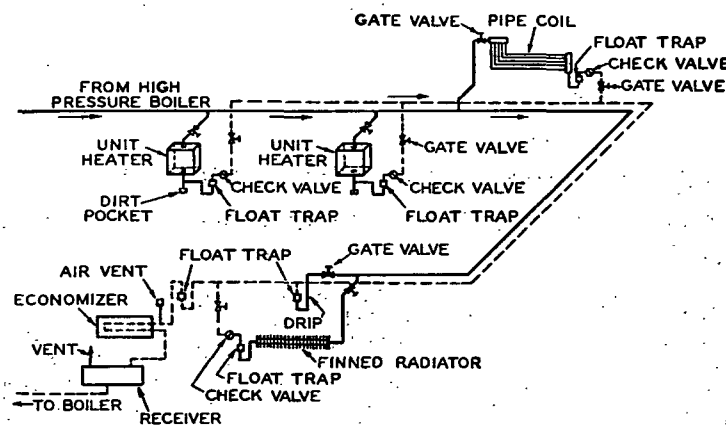
FIG. 8. TYPICAL HIGH PRESSURE HEATING SYSTEM
